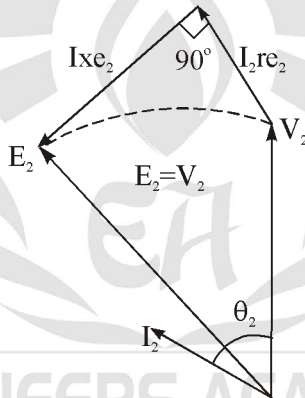
Figure : Phasor Diagram for 1-φ transformer for zero V.R.
